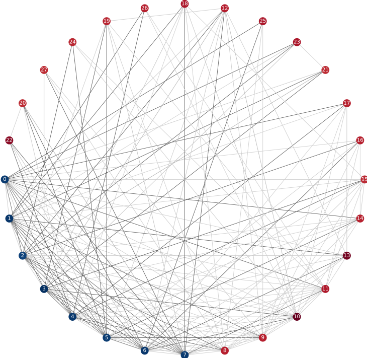
Fig. 4.2. Representation of f(t_i) = (t_1^2 + t_2^2 - 149)^2 as a quadratized Ising model. Nodes, corresponding to spins, can be arranged in a circle and are quadratically coupled by links. Weaker couplings are represented in light grey, gradually getting darker for higher coupling strengths. Linear couplings are coloured from dark blue (large negative terms) to dark red (large positive terms).
