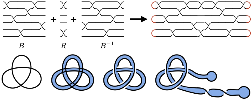
Fig. 8.8. Generating ribbon knots. Top: SYM algorithm. Bottom: UNSYM algorithm.
