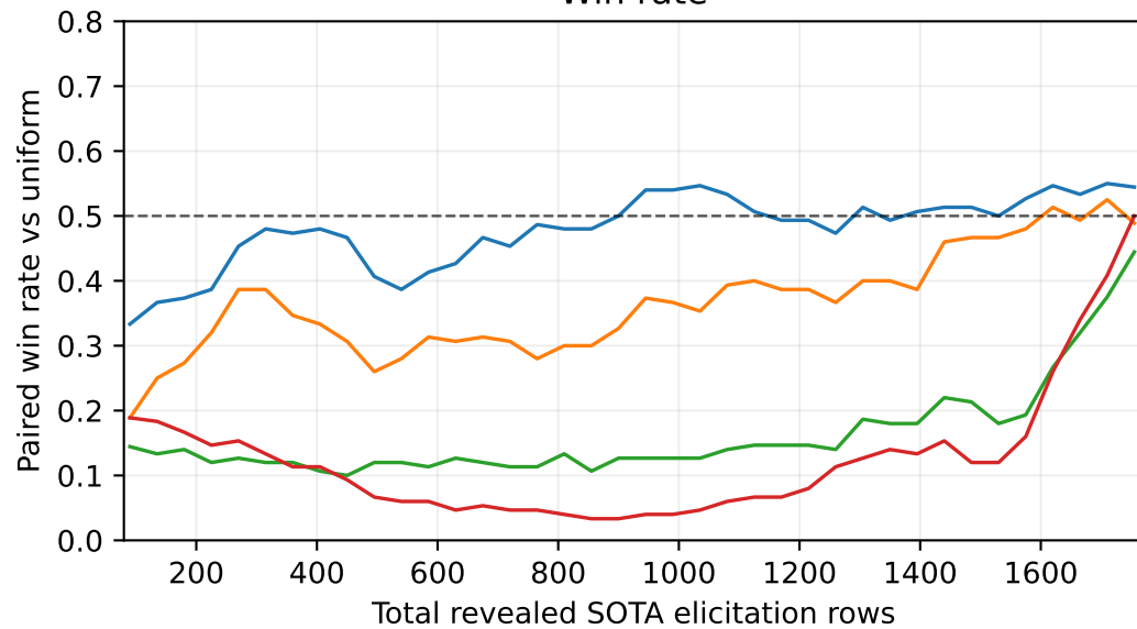
Win rate
