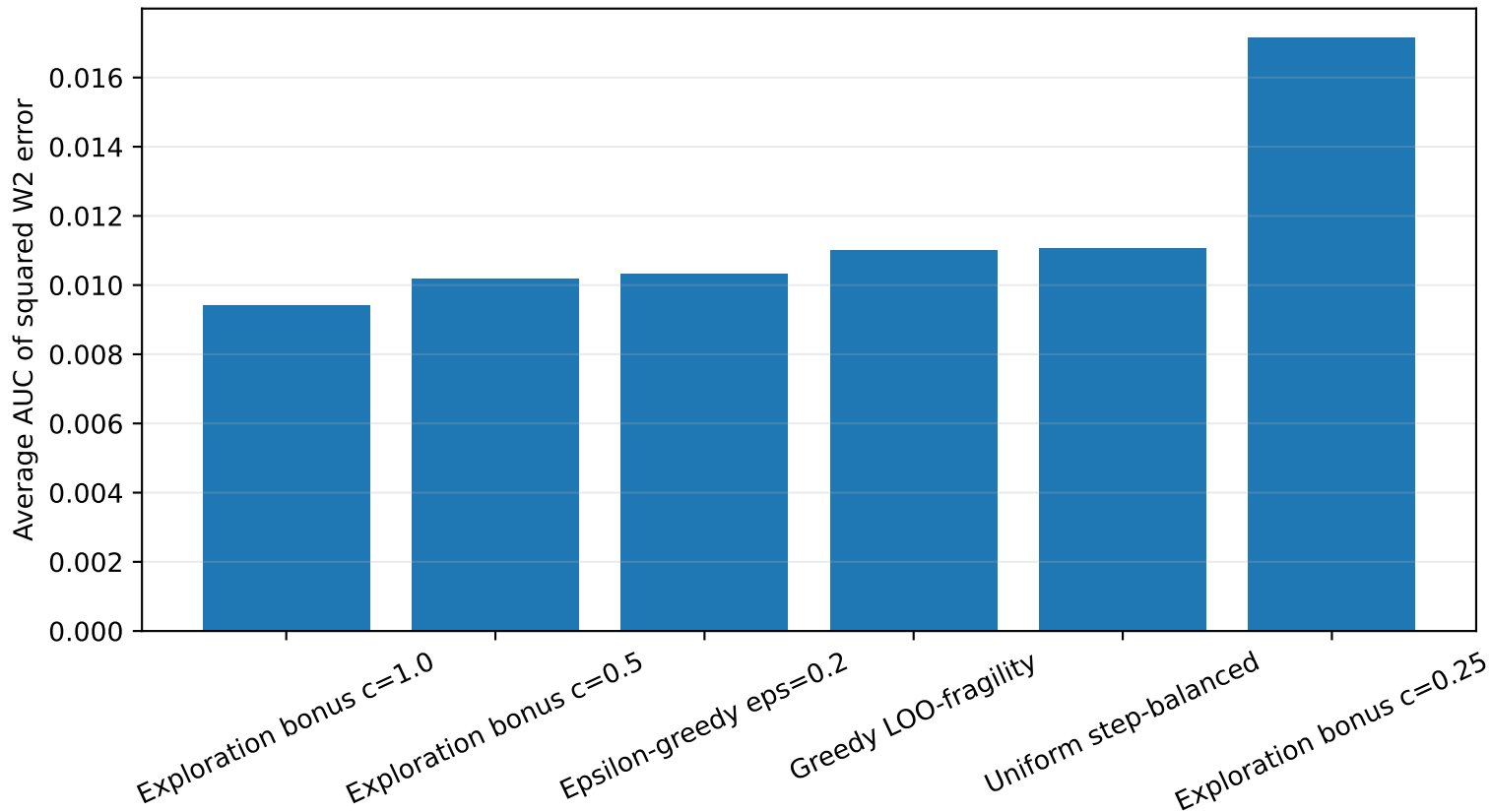
Locked Hidden-Reveal AUC by Policy
