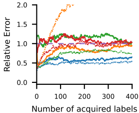
70B-few
