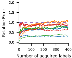
7B-few
