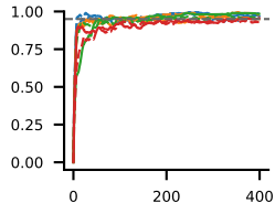
Coverage probability
