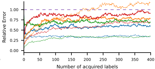
Gemma3-4b-few
