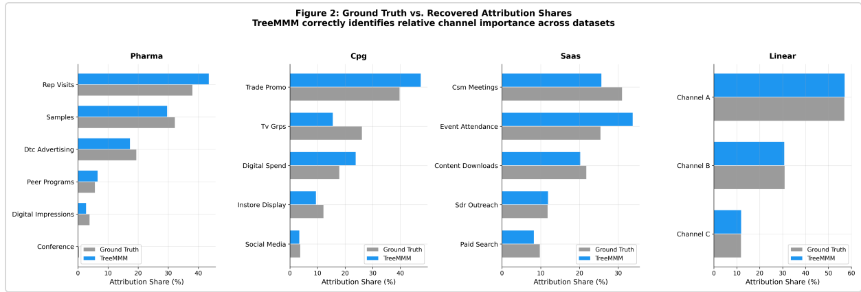
Figure 2. Attribution shares per channel. Reference shares (gray) versus TreeMMM-recovered shares (blue) for each channel within each dataset, after promo-only renormalization.
