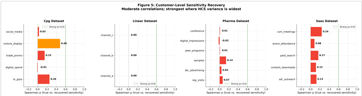
Figure 5. Heterogeneous customer sensitivity recovery. Spearman rho between true latent per-customer sensitivity and recovered mean absolute SHAP, by channel and dataset.
