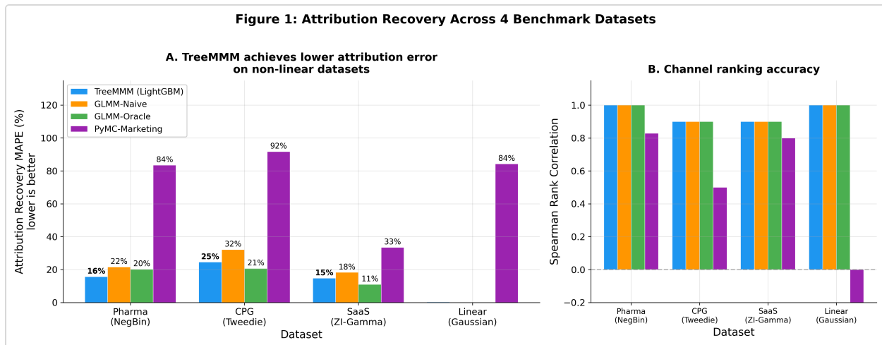
Figure 1. Attribution recovery across four benchmark DGPs. Left: share-MAPE between recovered and reference channel shares (lower is better). TreeMMM (blue) achieves lower share-MAPE than GLMM-Naive (orange) on all three non-linear datasets. Right: Spearman rank correlation between recovered and true channel rankings.
