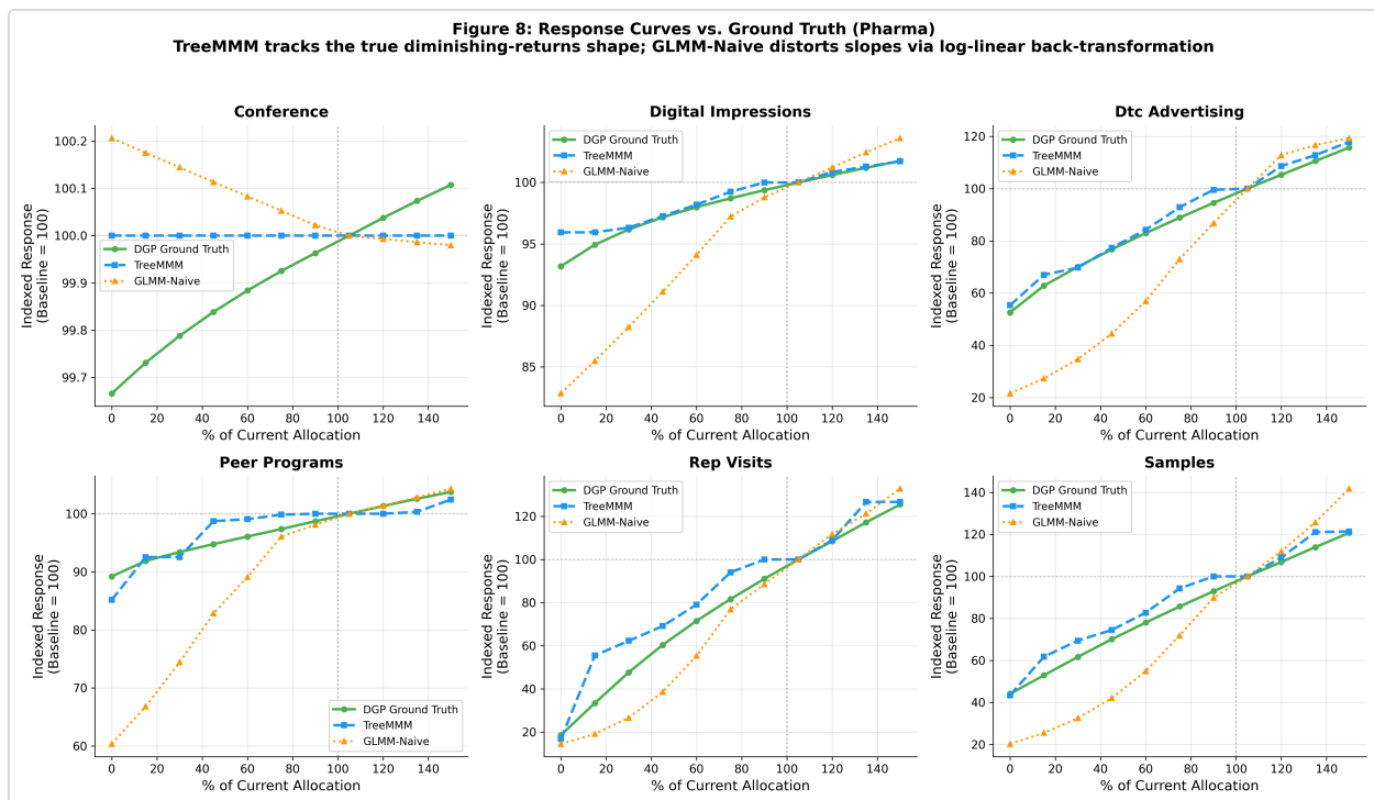
Figure 8. Normalized response curves on the pharma DGP. Each panel shows one channel; curves are indexed to 100 at baseline allocation for shape comparison. DGP ground truth (green), TreeMMM (blue), GLMM-Naive (orange).
