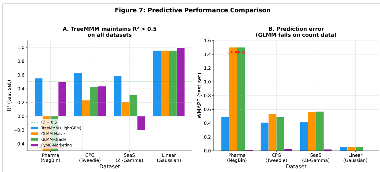
Figure 7. Predictive performance on held-out test folds. Left: R-squared per dataset and model. Right: weighted MAPE on response-scale predictions.
