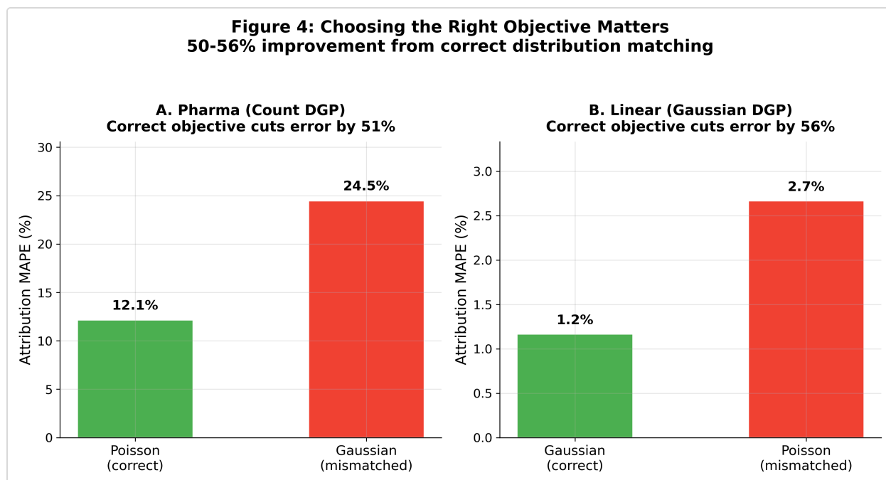
Figure 4. Distribution-aware objective selection. Share-MAPE under the correct objective (green) versus a mismatched Gaussian objective (red) on the pharma DGP, and the mirror comparison on the linear DGP. Correct objective selection reduces share-MAPE by roughly 50 to 56 percent.
