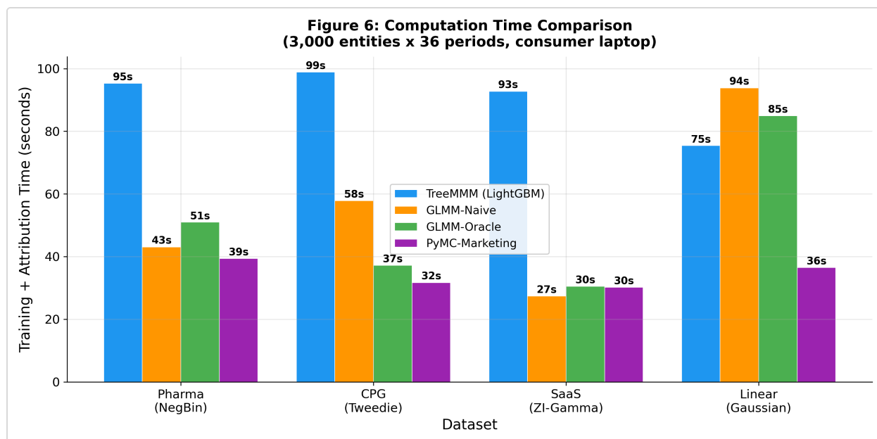
Figure 6. Computation time per dataset for training and attribution. All methods complete within 100 seconds on a consumer laptop at the 3,000 by 36 benchmark scale.
