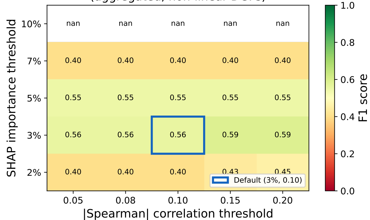
B. F1 heat-map (aggregated, non-linear DGPs)
