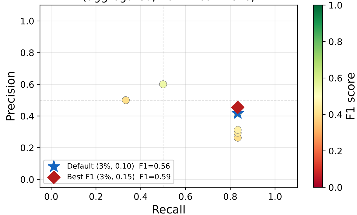
A. Precision-Recall landscape (aggregated, non-linear DGPs)
