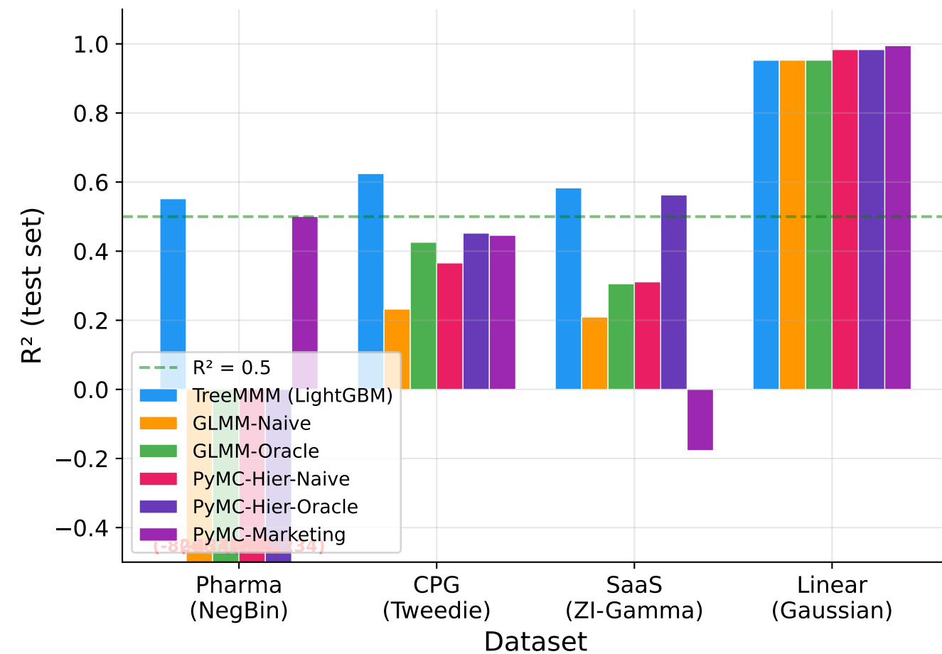
A. TreeMMM maintains R^2 > 0.5 on all datasets
