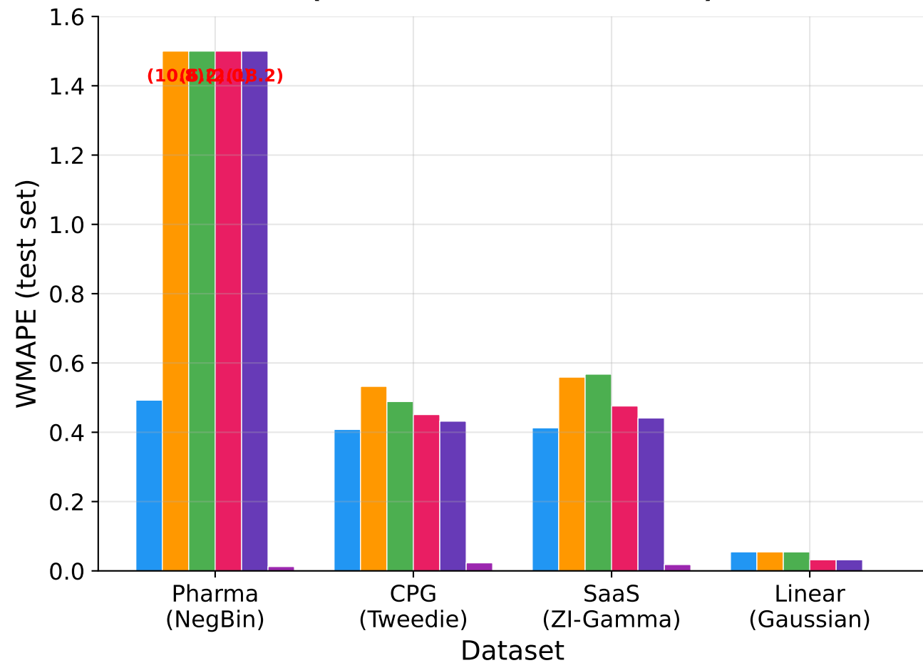
B. Prediction error (GLMM fails on count data)
