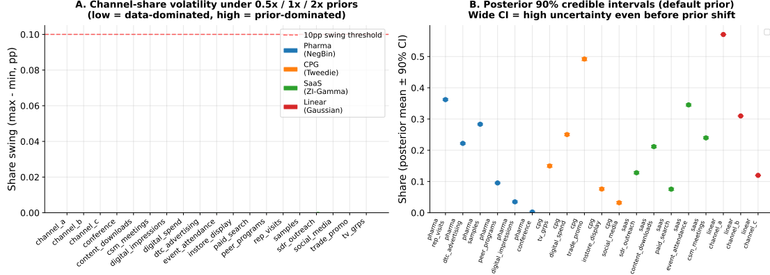
Figure 12: Bayesian prior sensitivity. Panel A: max-minus-min channel-share swing across prior scales 0.5\times , 1\times , 2\times for each (dataset, channel) combination, with a 10 pp reference line. Panel B: posterior 90% credible interval per channel at the default prior.
