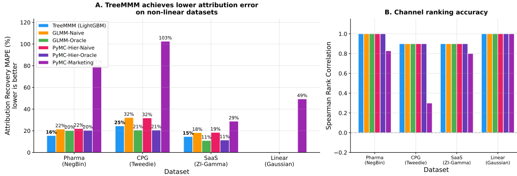
Figure 1: Attribution Recovery Across 4 Benchmark Datasets
