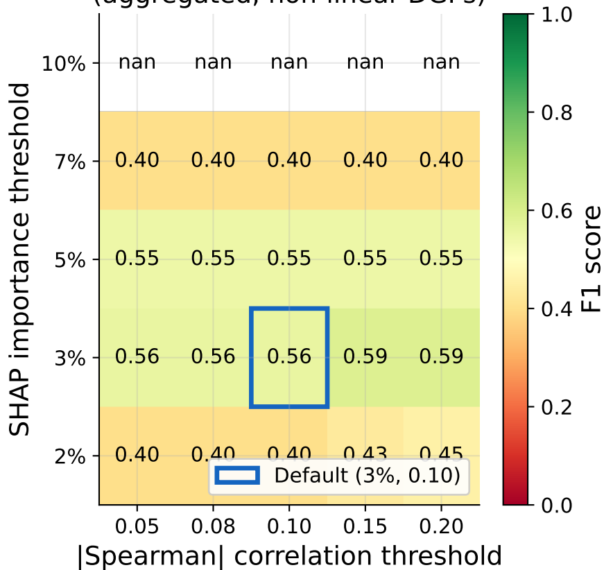
B. F1 heat-map (aggregated, non-linear DGPs)
