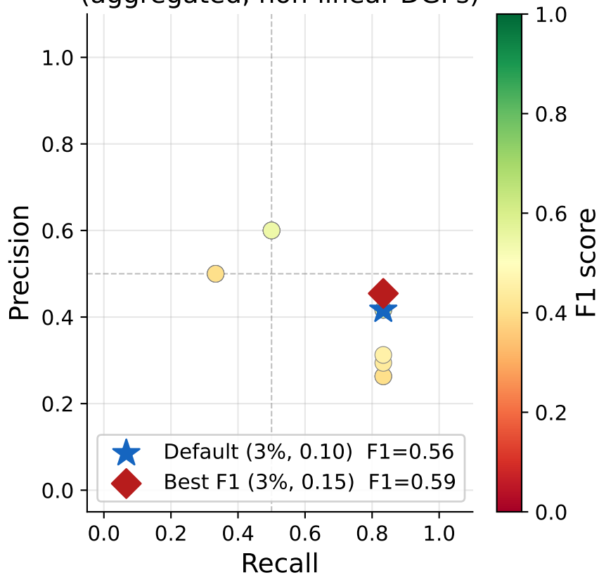
A. Precision-Recall landscape (aggregated, non-linear DGPs)
