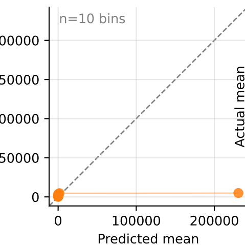
GLMM-Naive
