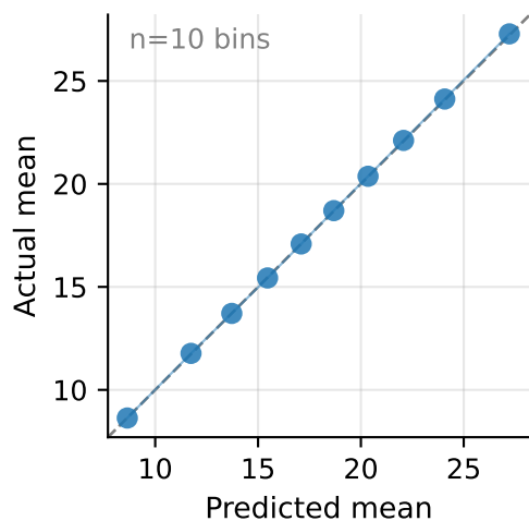
Linear (Gaussian)
