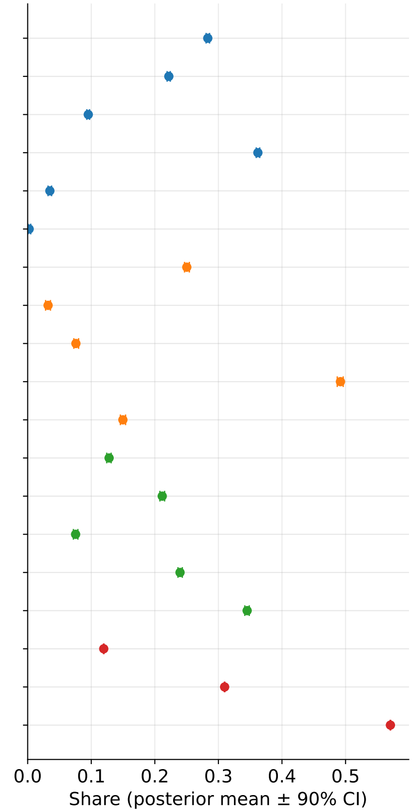
B. Posterior 90% credible intervals (default prior) Wide CI = high uncertainty before prior shift
