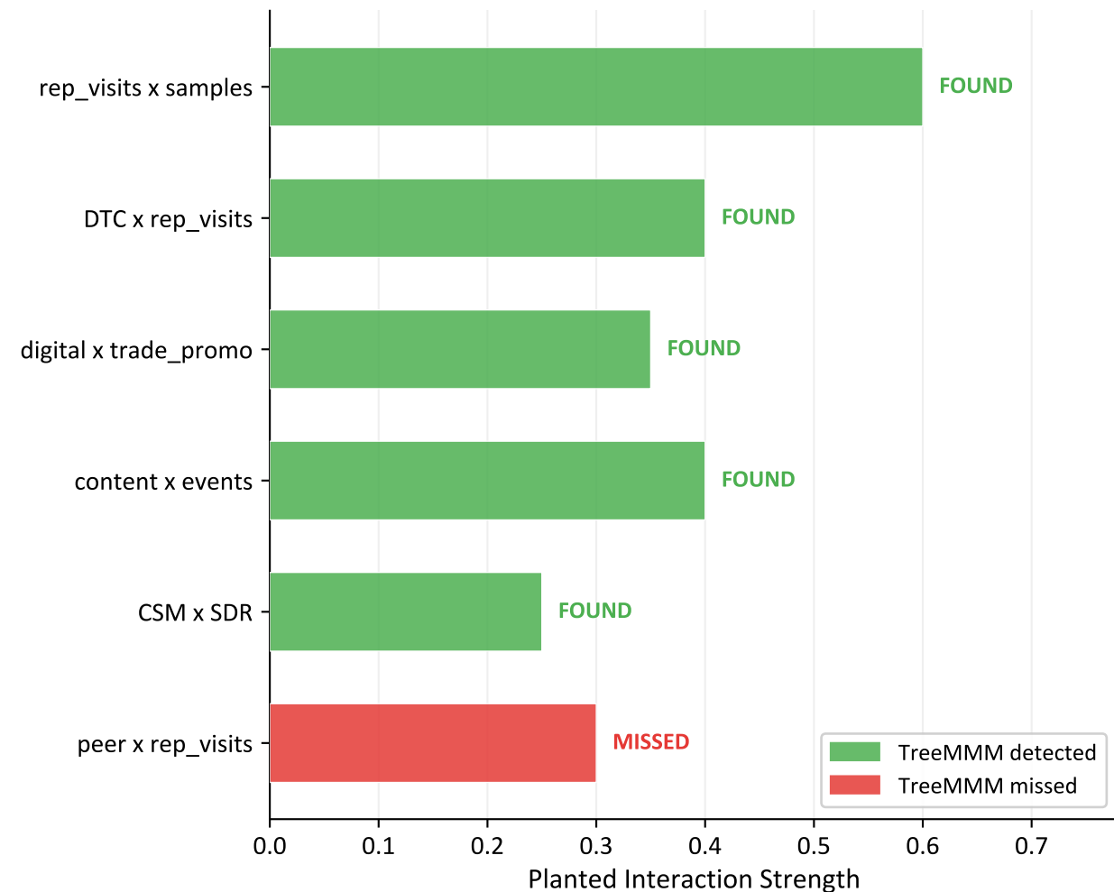
5 of 6 Interactions Found Automatically (regression finds 0/6 without manual specification)
