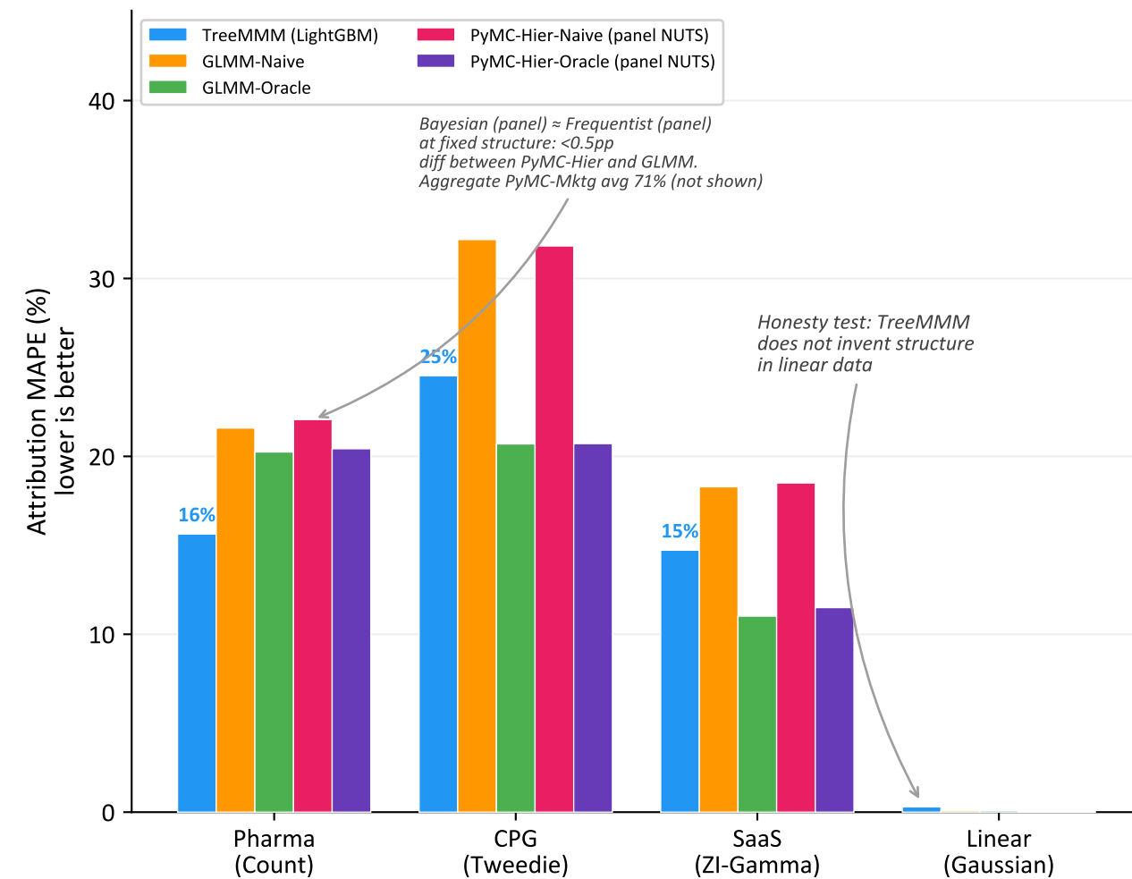
Customer-Level (Panel) Comparison TreeMMM within 1–6pp of Oracle; 6pp ahead of Naive baselines
