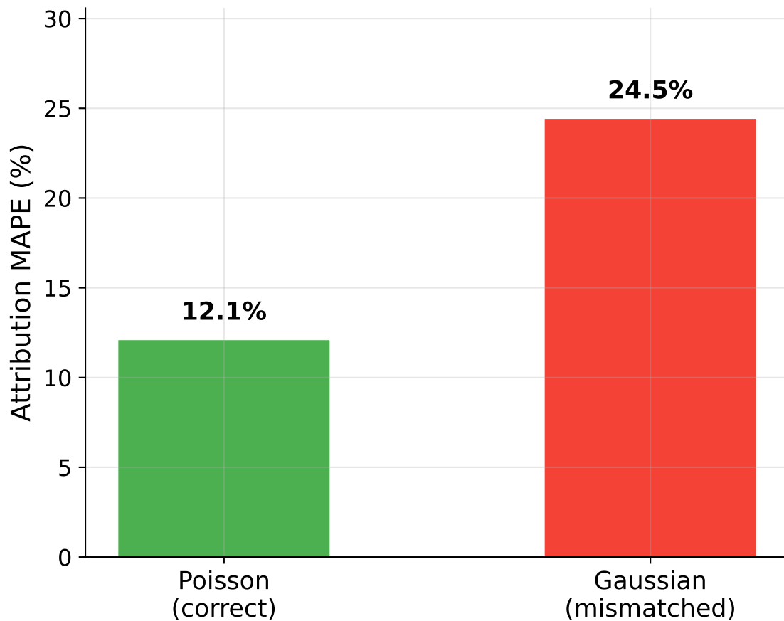
A. Pharma (Count DGP) Correct objective cuts error by 51%
