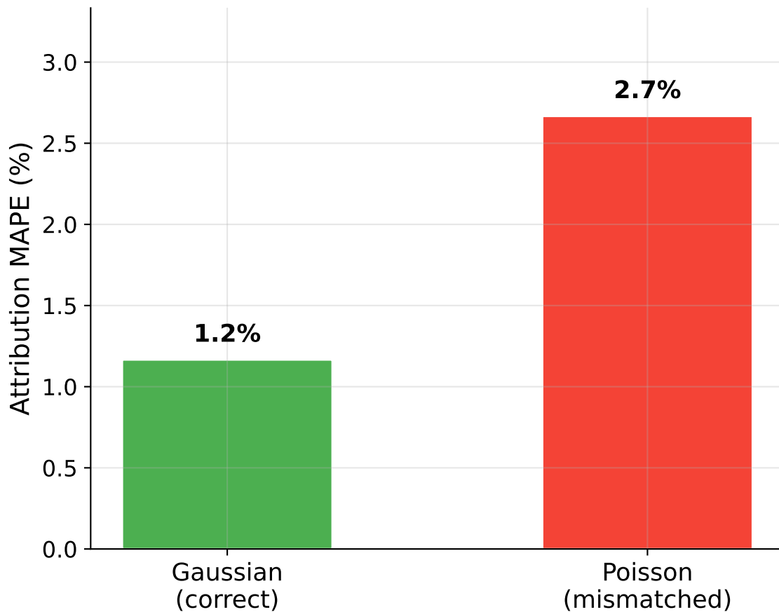
B. Linear (Gaussian DGP) Correct objective cuts error by 56%
