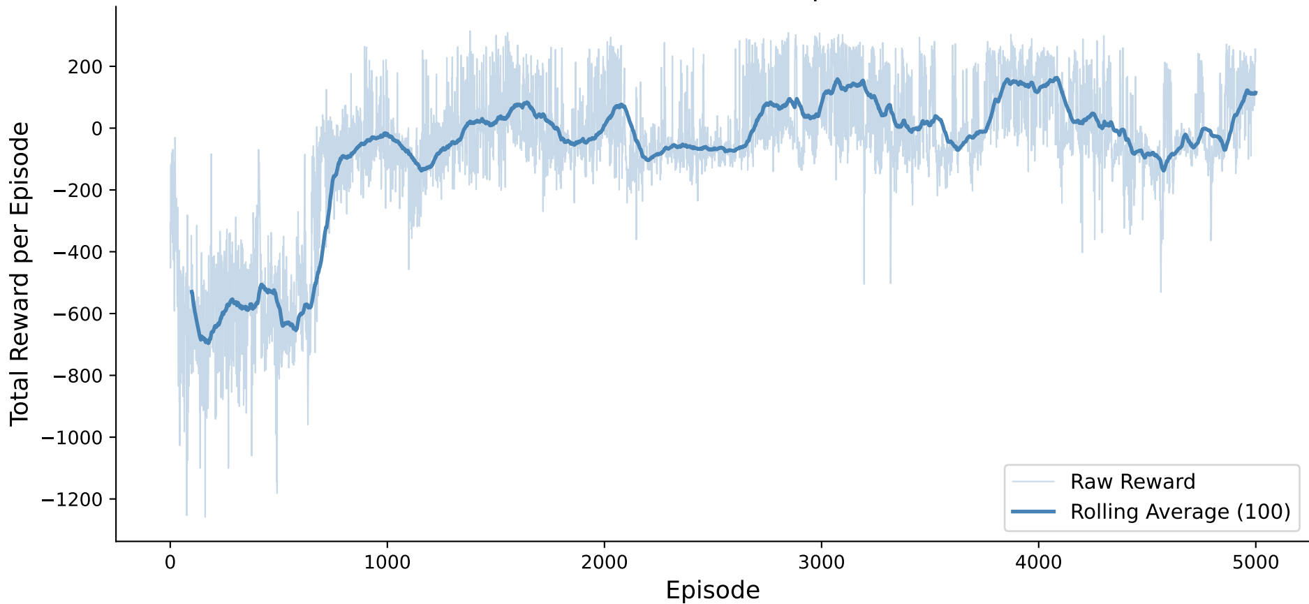
A2C — Reward over Episodes
