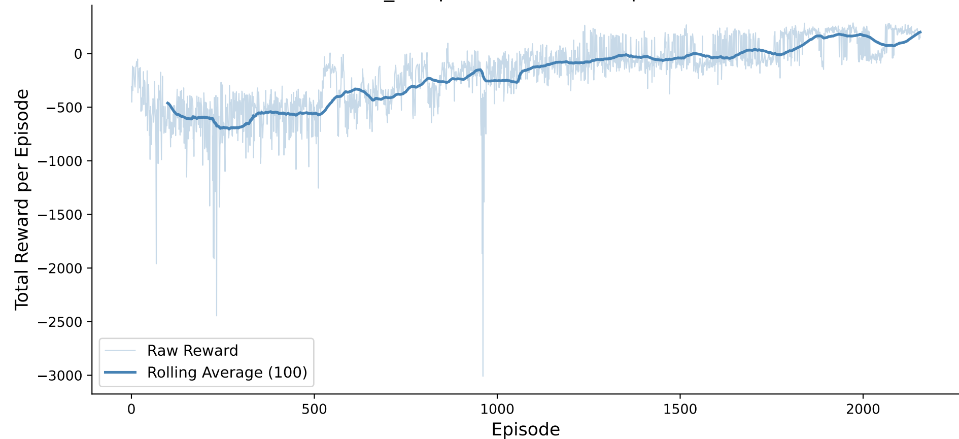
A2C_nstep — Reward over Episodes
