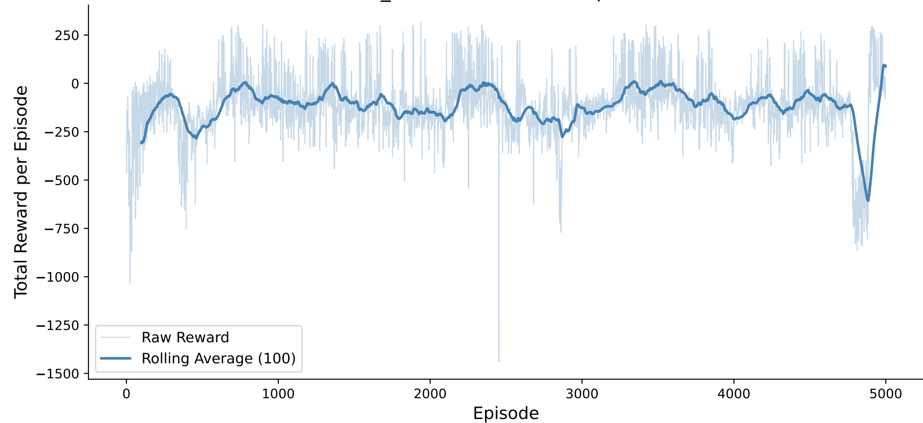
A2C_td1 — Reward over Episodes
