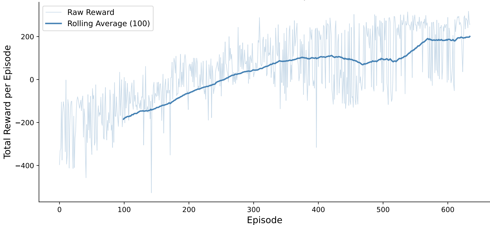
DQN — Reward over Episodes
