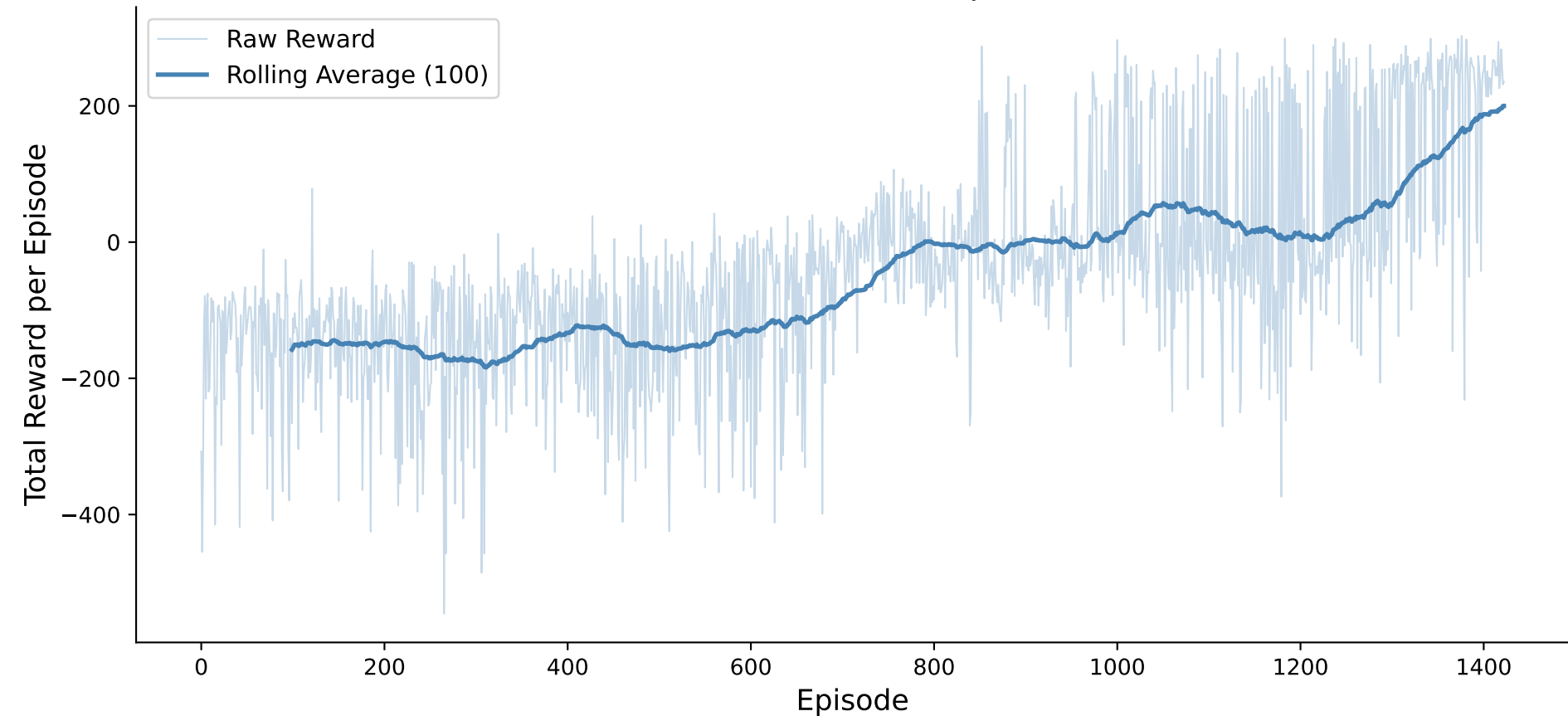
PPO — Reward over Episodes
