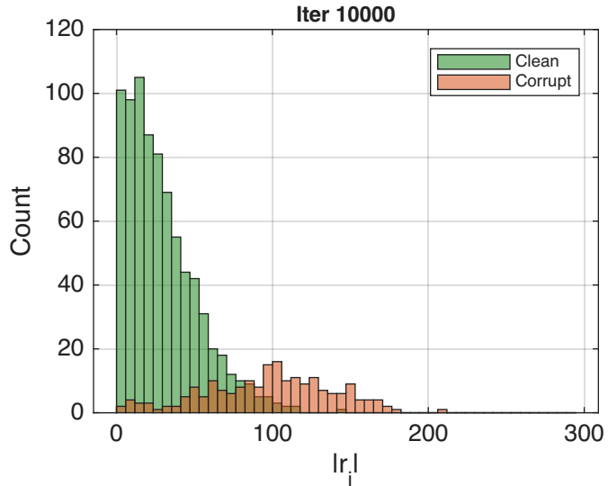
Gaussian N(0,1) — Residual Histograms: QRK q 0.90
