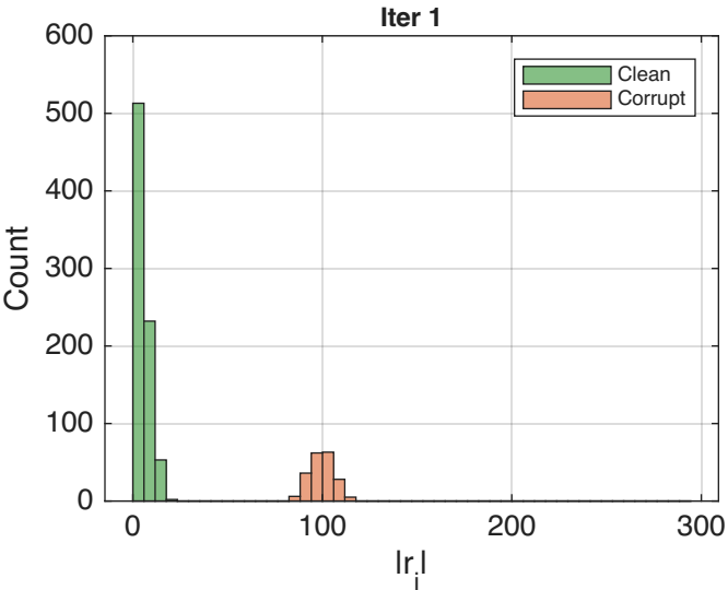
Gaussian N(0,1) — Residual Histograms: QRK q 0.90
