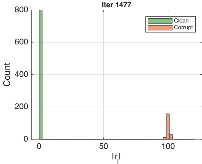
Gaussian N(0,1) — Residual Histograms: constant t_{\text{hresh}}
