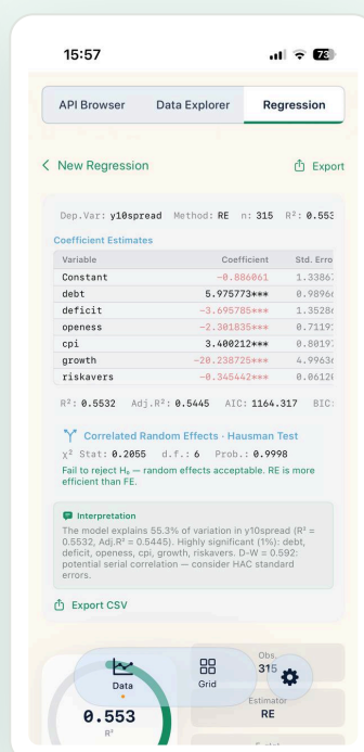
Model results with built-in interpretation
