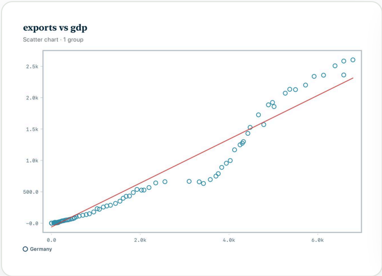
Publication-ready scatter plot with fitted relationship
