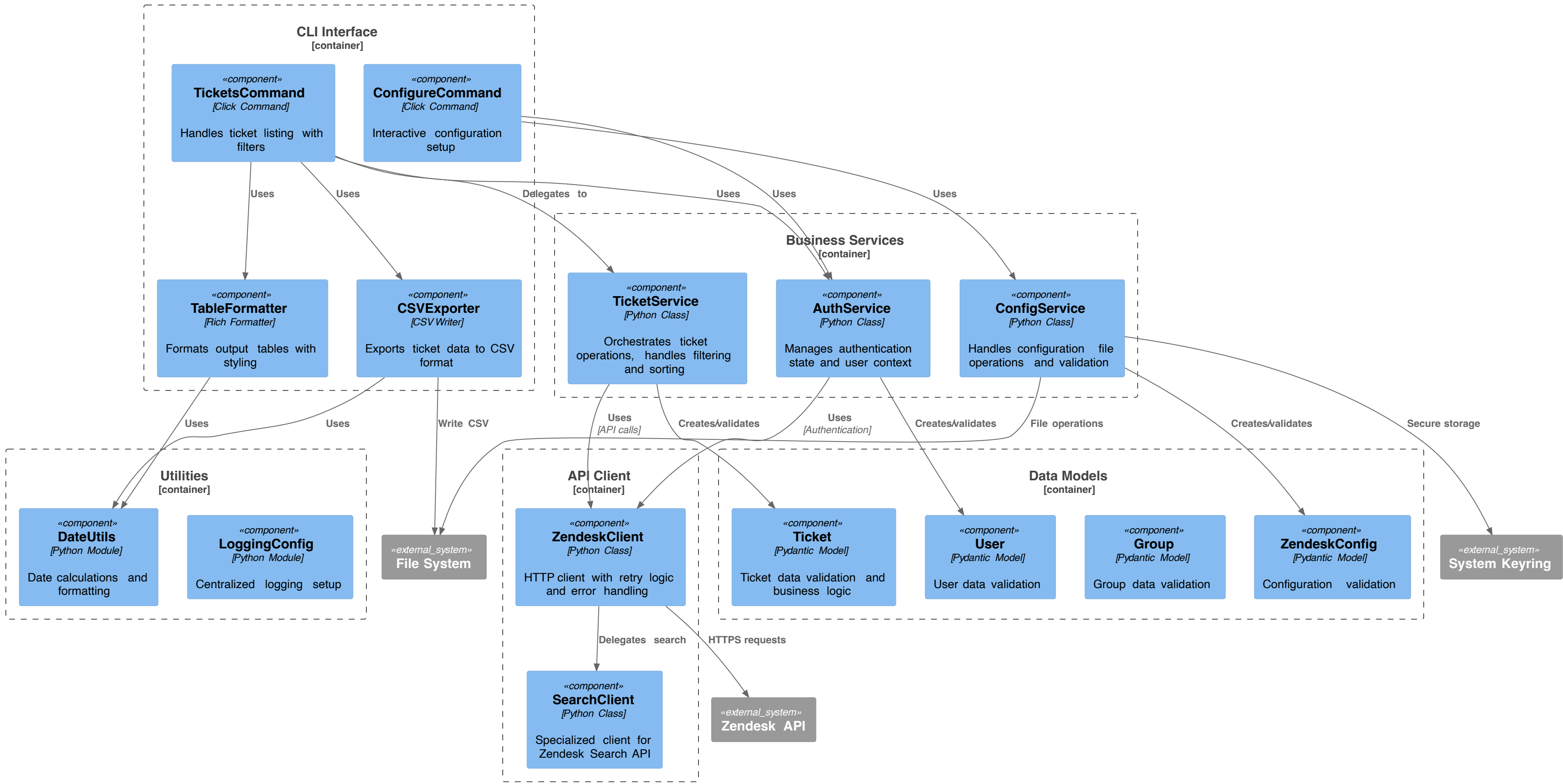
Component Diagram - Business Services Layer
