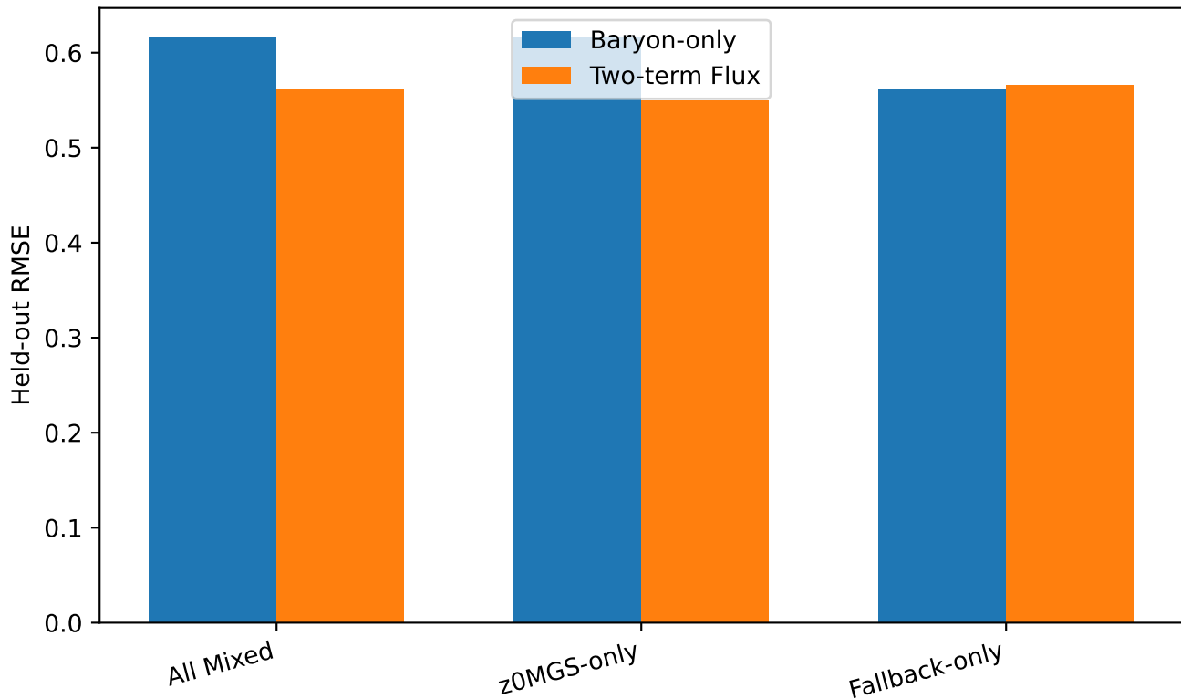
3-mode empirical SFH cross-validation
