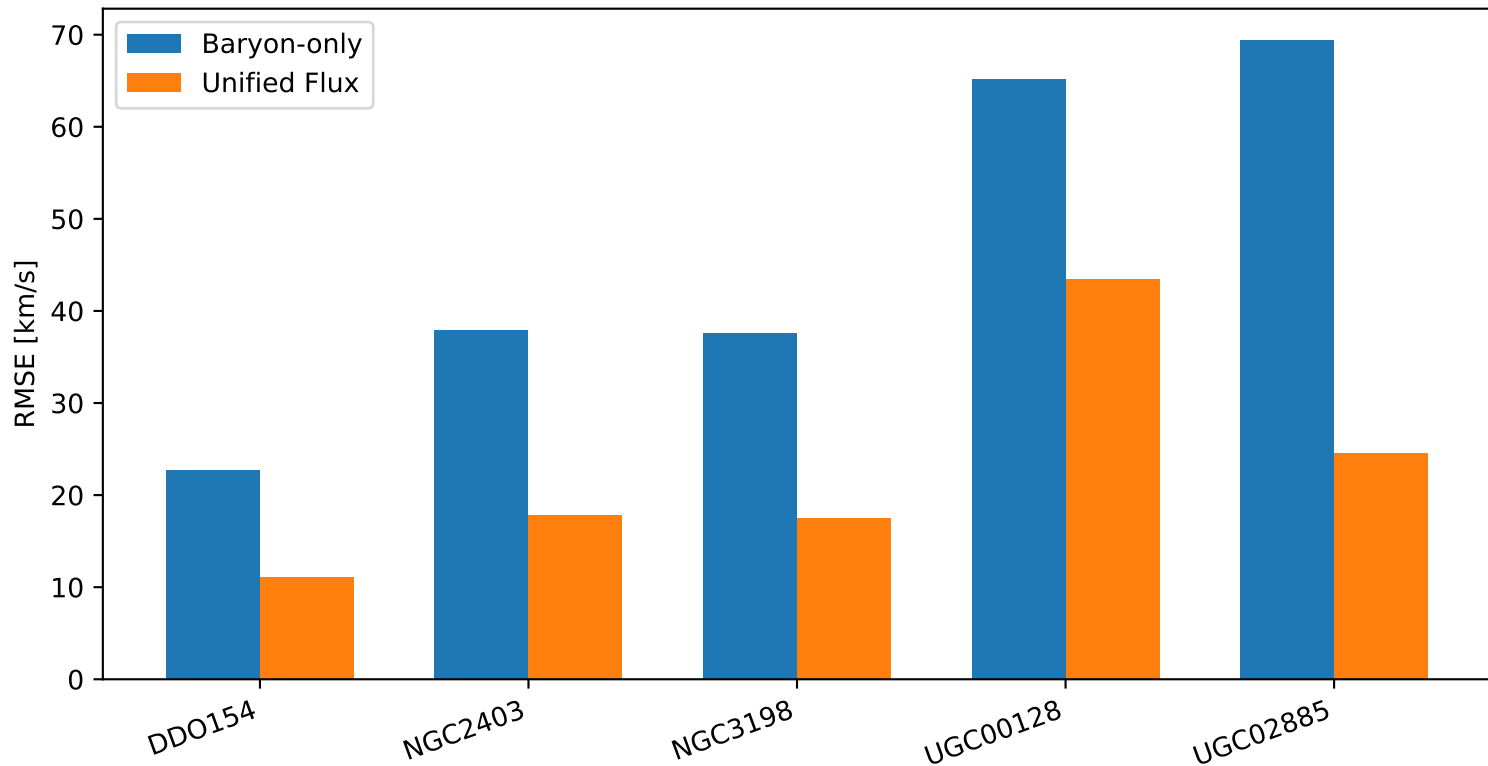
Unified radial benchmark on five SPARC galaxies
