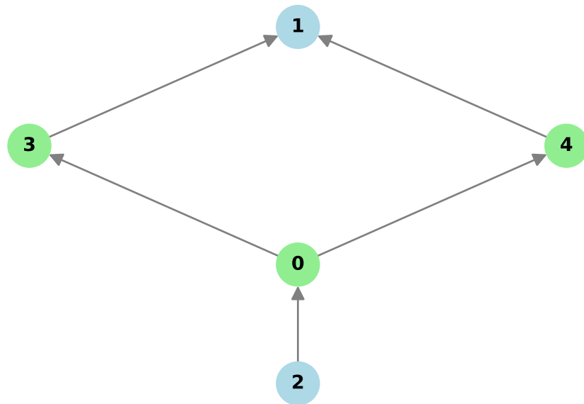
Lattice
