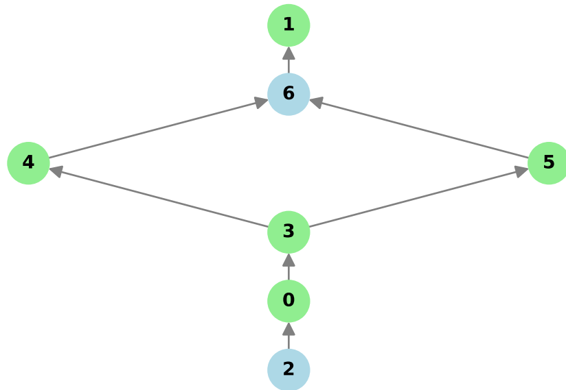
Lattice
