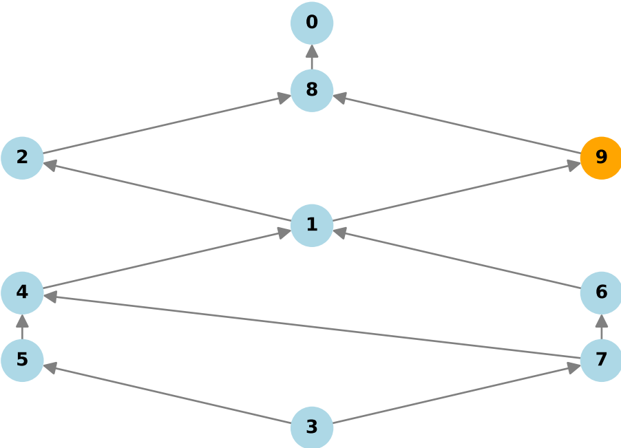
Fusion SemiLattice
