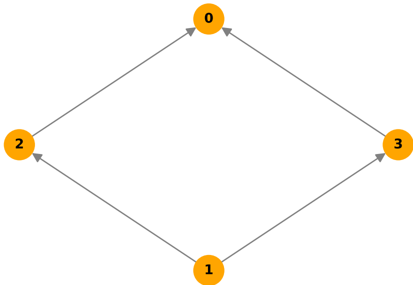
Fusion SemiLattice
