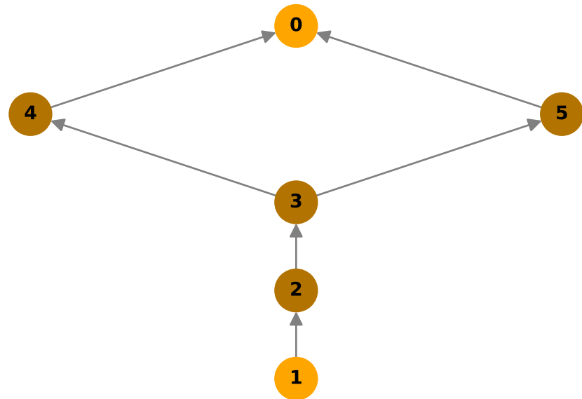
Join Lattice
