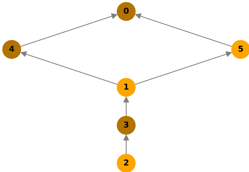
Fusion SemiLattice
