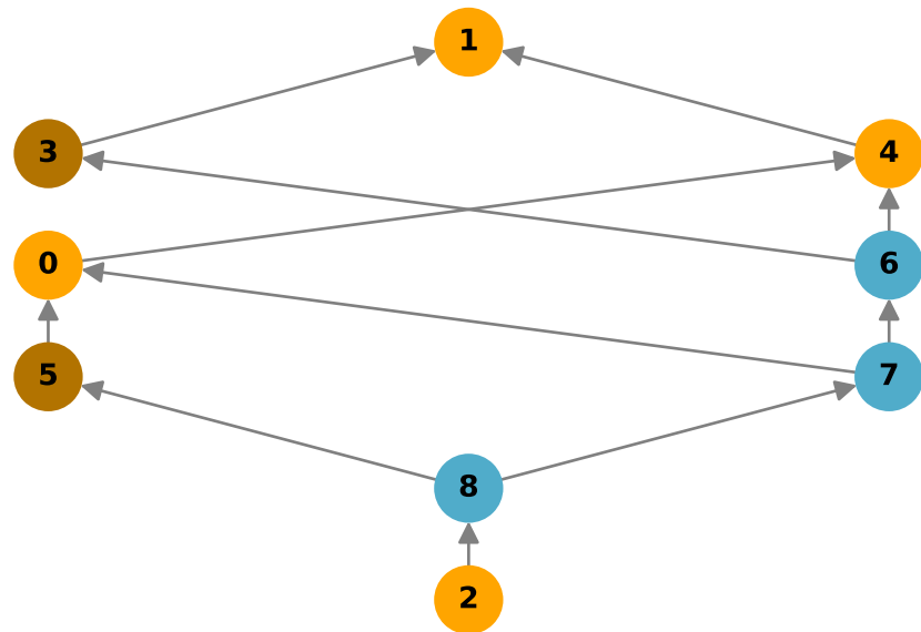
Join Lattice
