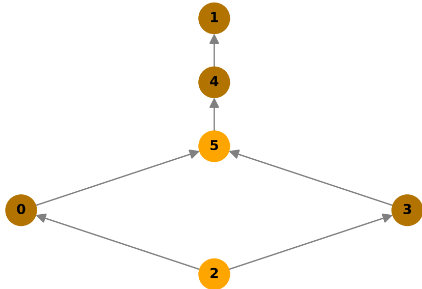
Join Lattice
