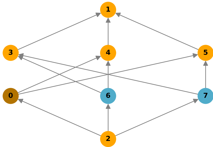
Join Lattice
