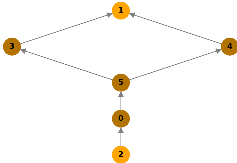
Join Lattice
