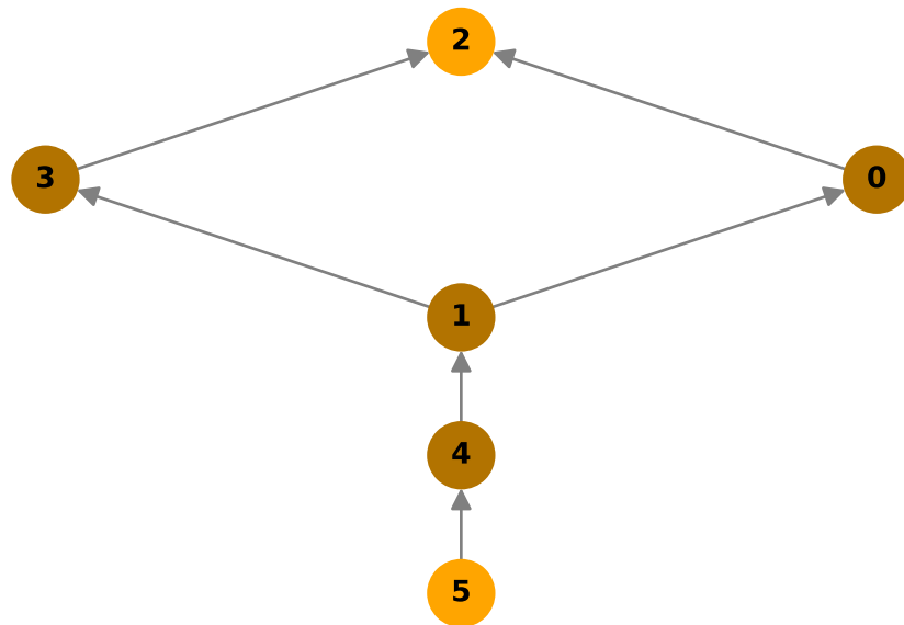
Join Lattice
