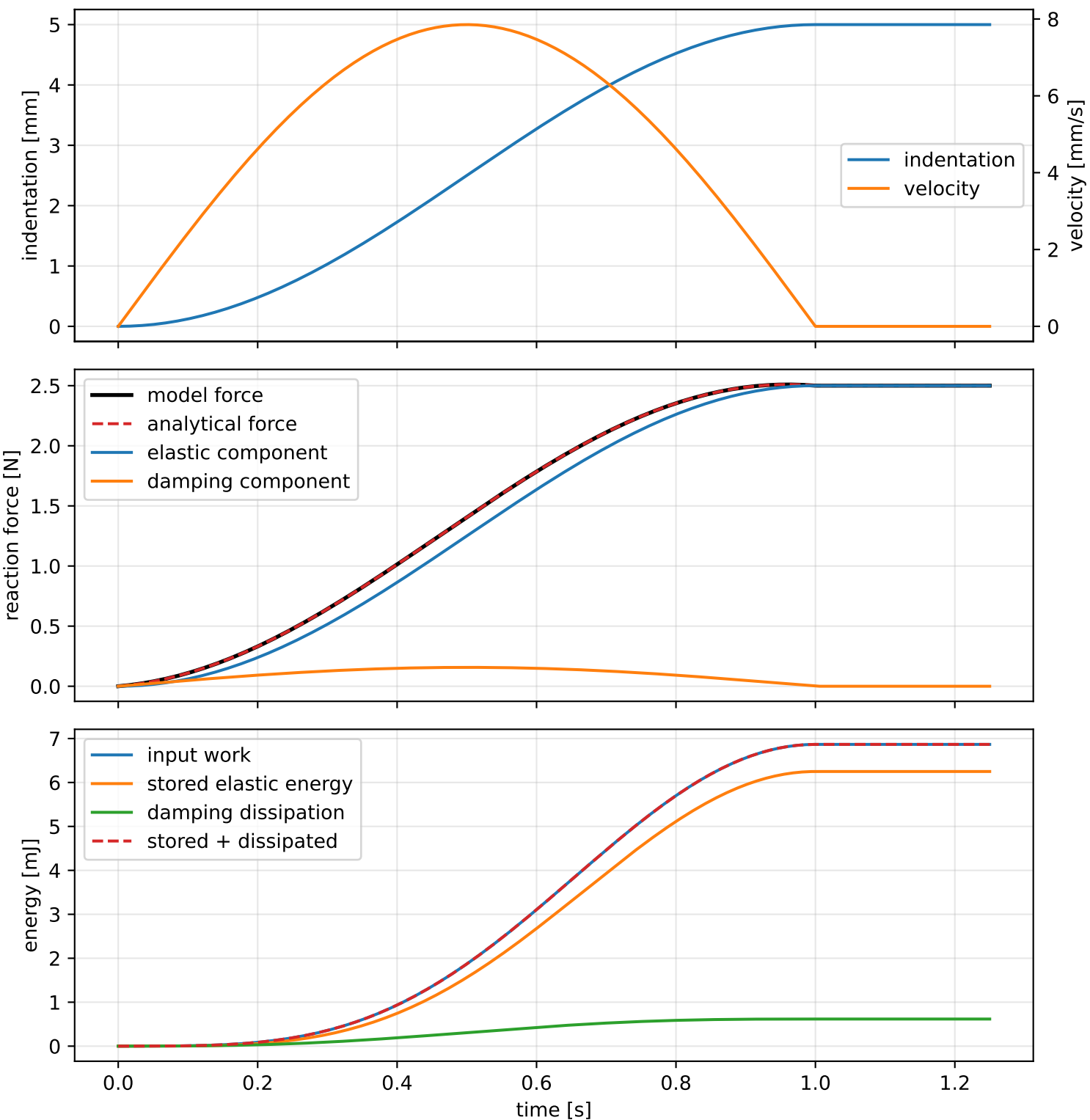
Kelvin-Voigt response to a bounded raised-cosine ramp
