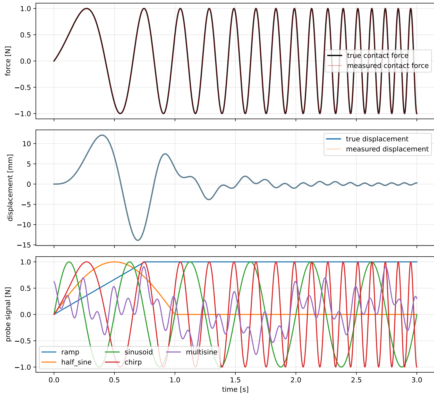
EXP-0001 time histories — near_ideal_compliant_chirp
