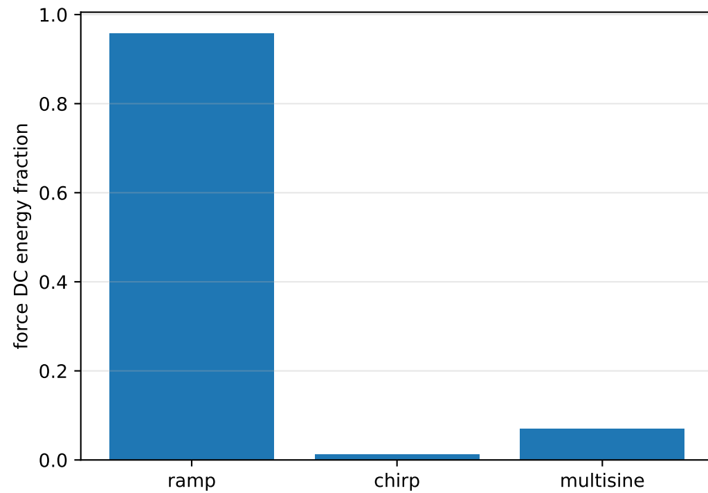
EXP-0001 ramp failure: static content and weak inertial excitation
