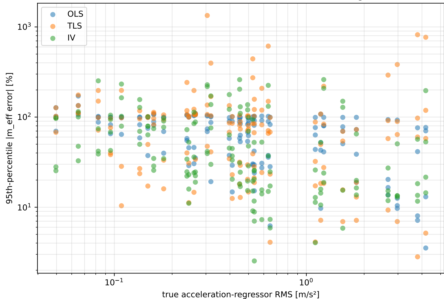
Effective-mass error versus inertial excitation strength
