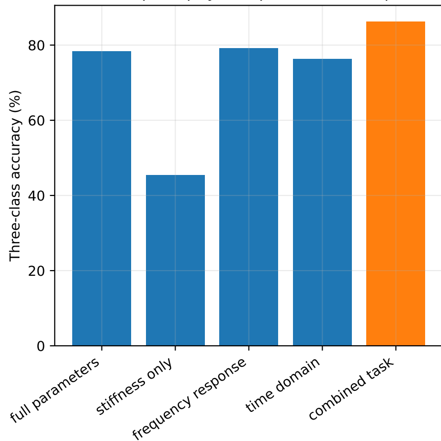
Do explicit physical parameters help?
