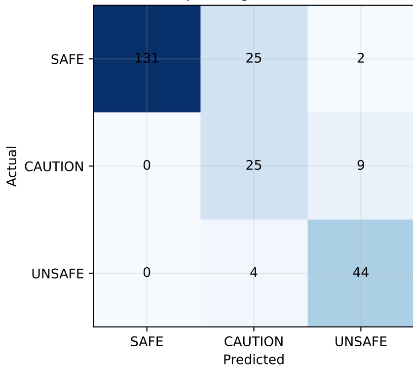
Nominal confusion matrices at matched probe energy Chirp features only Chirp + ring-down (0.5 s)
