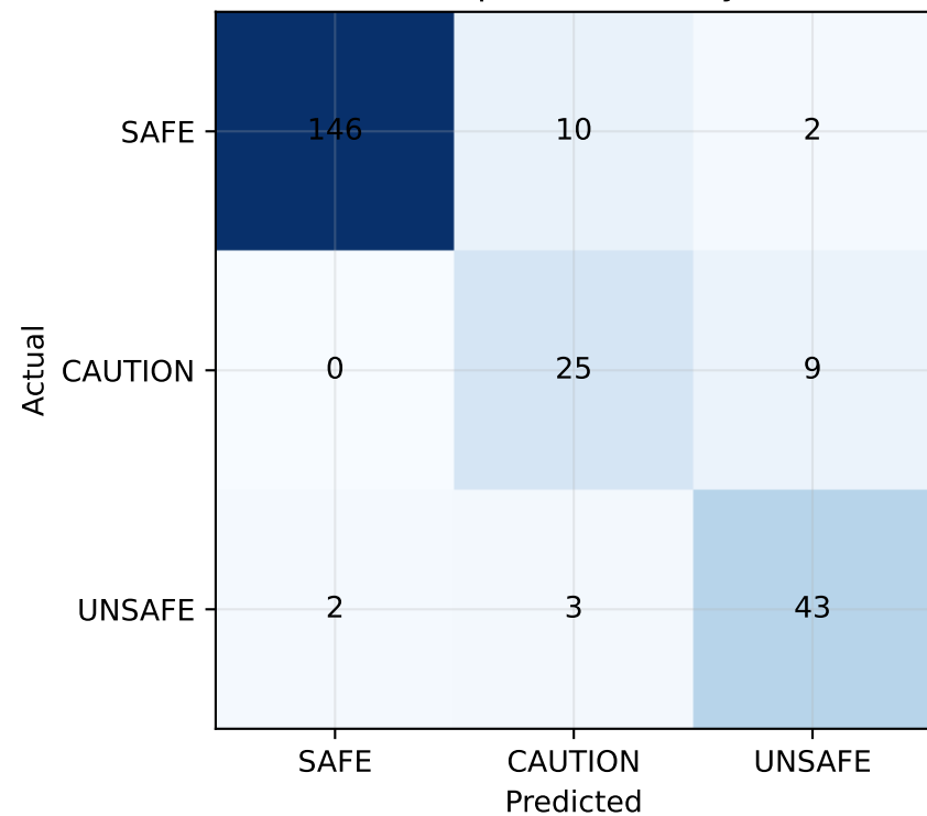
Nominal confusion matrices at matched probe energy Chirp features only Chirp + ring-down (0.5 s)
