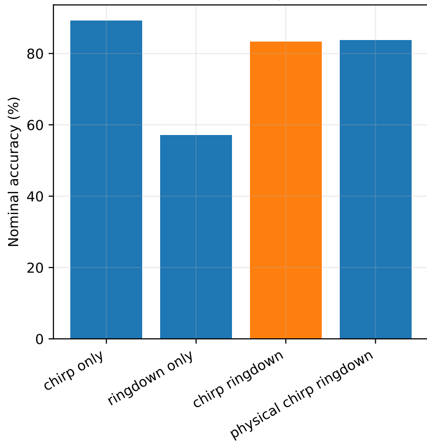
Feature-set comparison
