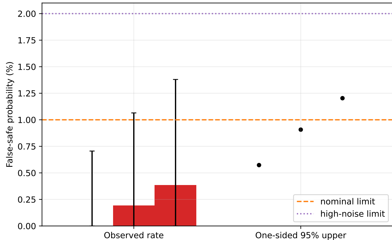
False-safe rate with binomial confidence bounds
