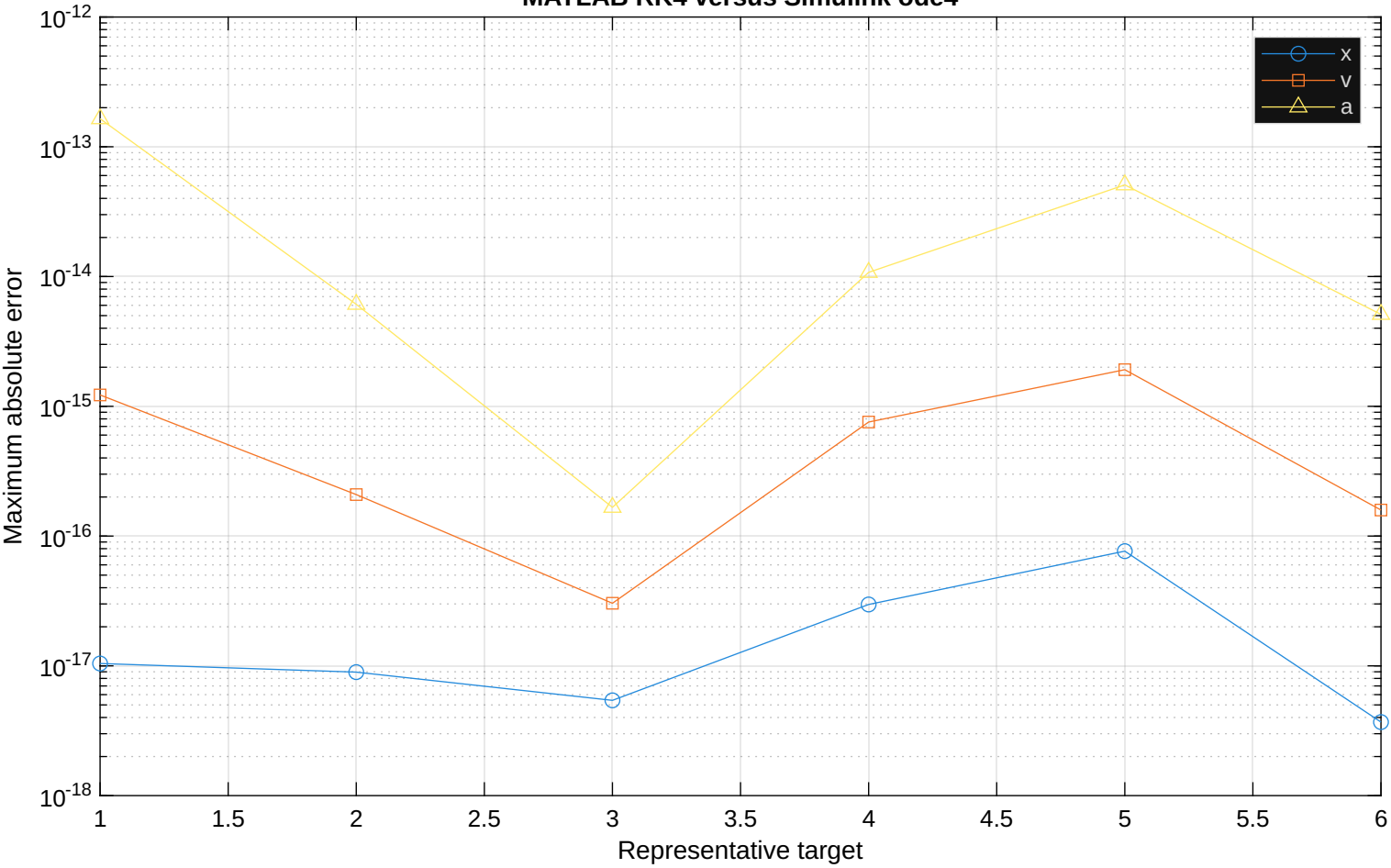
MATLAB RK4 versus Simulink ode4
