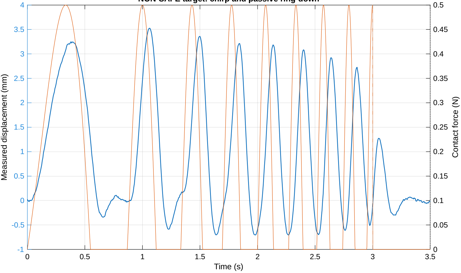
NON-SAFE target: chirp and passive ring-down
