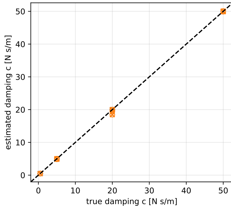
True versus estimated interaction parameters
