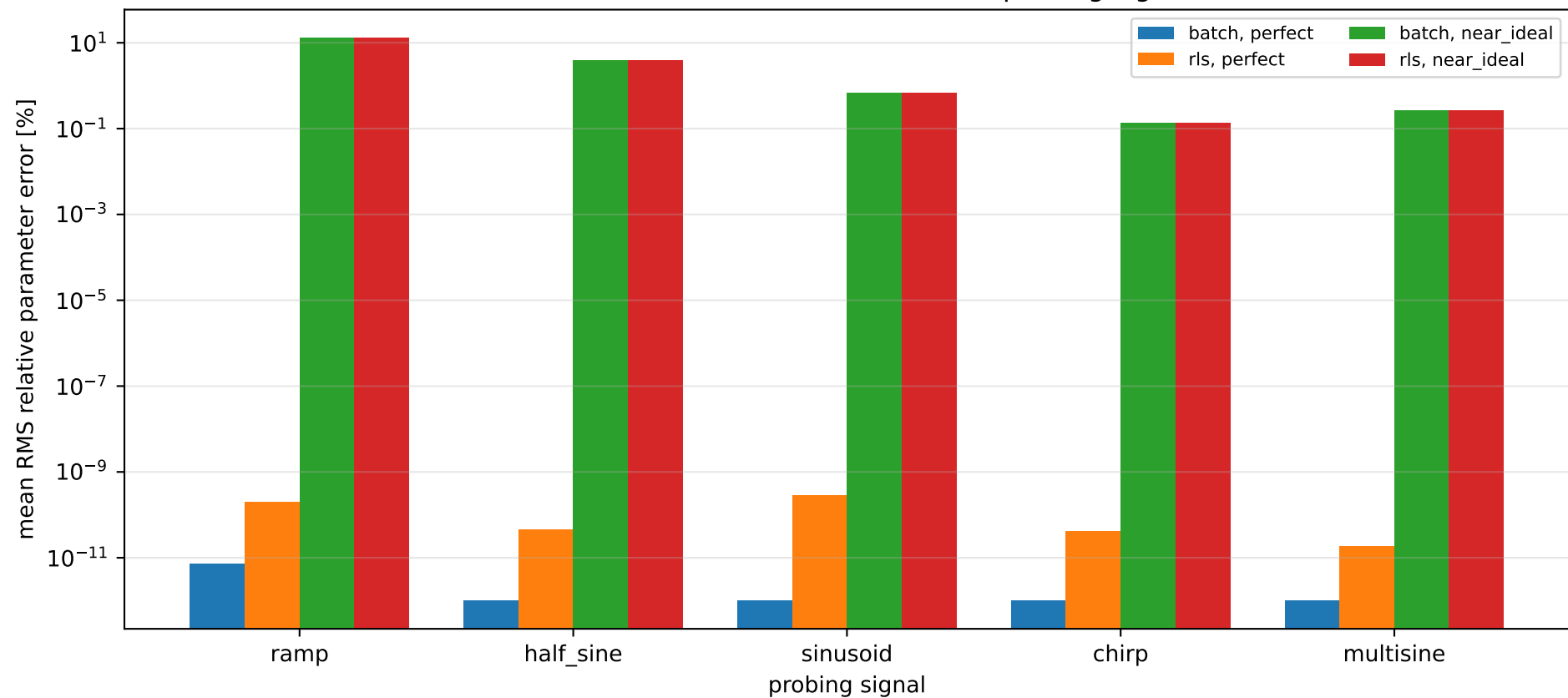
Identification error for each bounded probing signal
