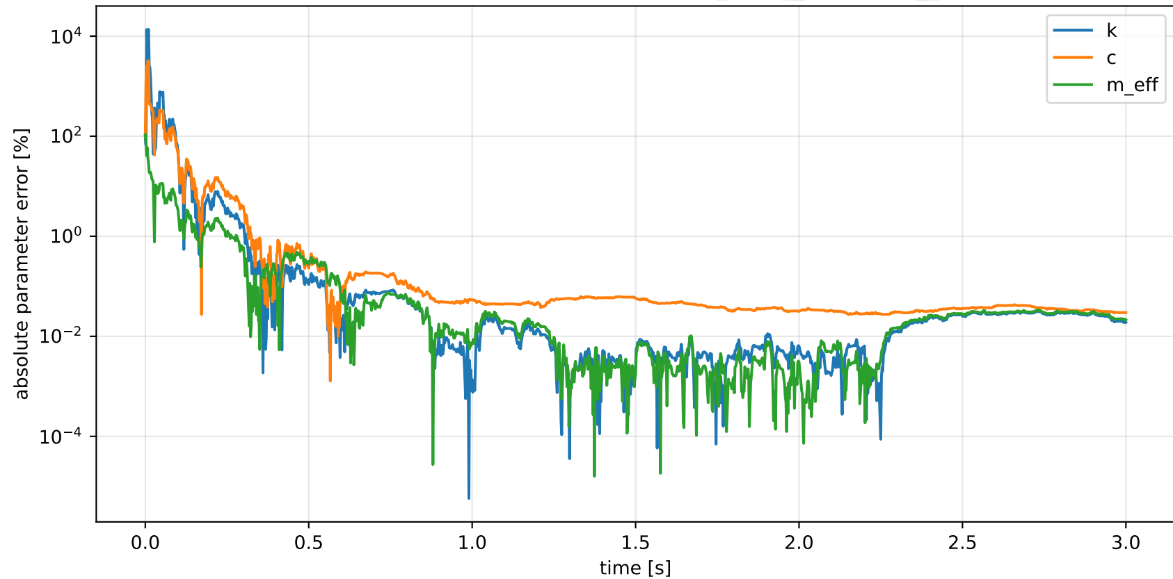
RLS parameter estimation error — near_ideal_compliant_chirp
