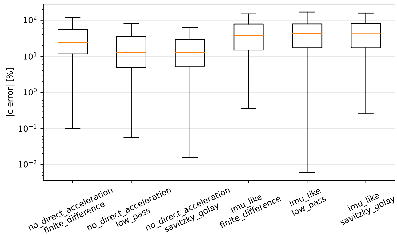
Parameter errors by practical measurement pipeline — nominal unilateral
