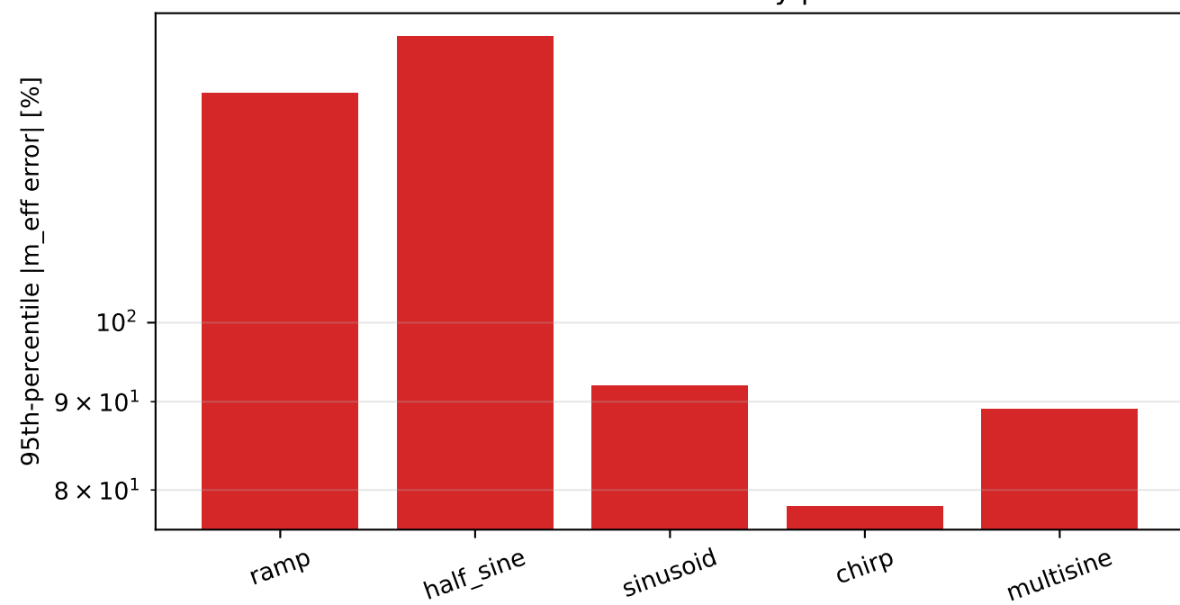
Effective-mass error by probe
