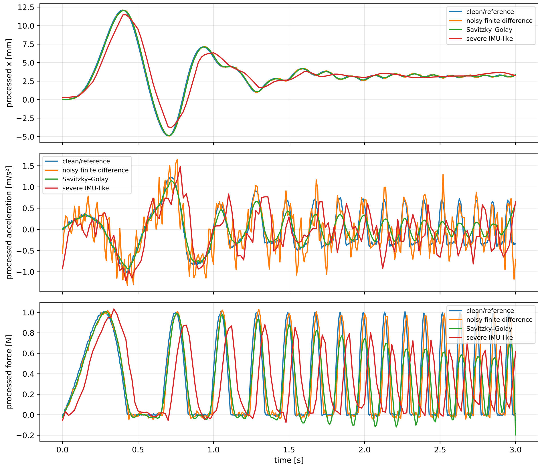
Representative clean, noisy, derived, and filtered signals
