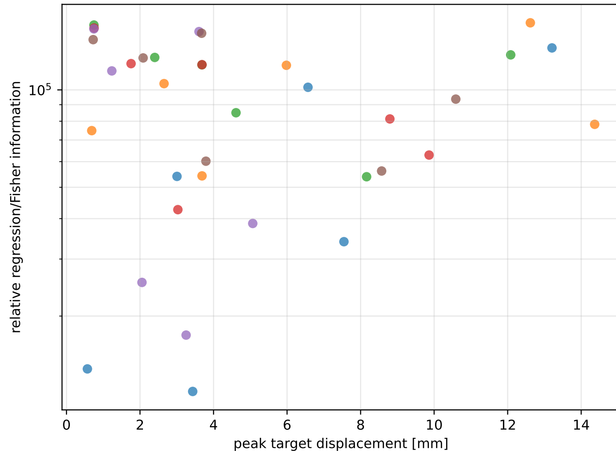
Information versus structural disturbance (fixed 1 N force bound)
