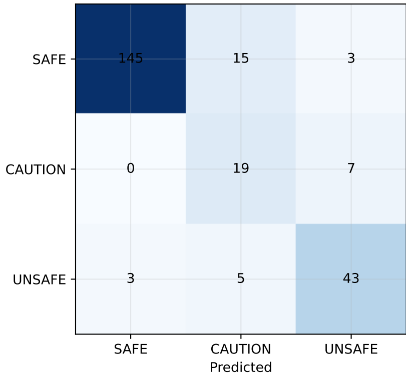
Nominal causal confusion matrix
