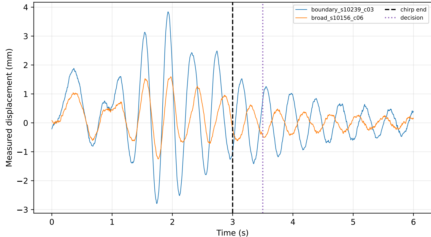
Observed false-safe cases (full response audit)
