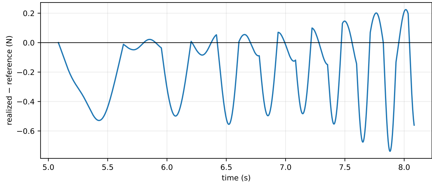
Probe force-tracking error
